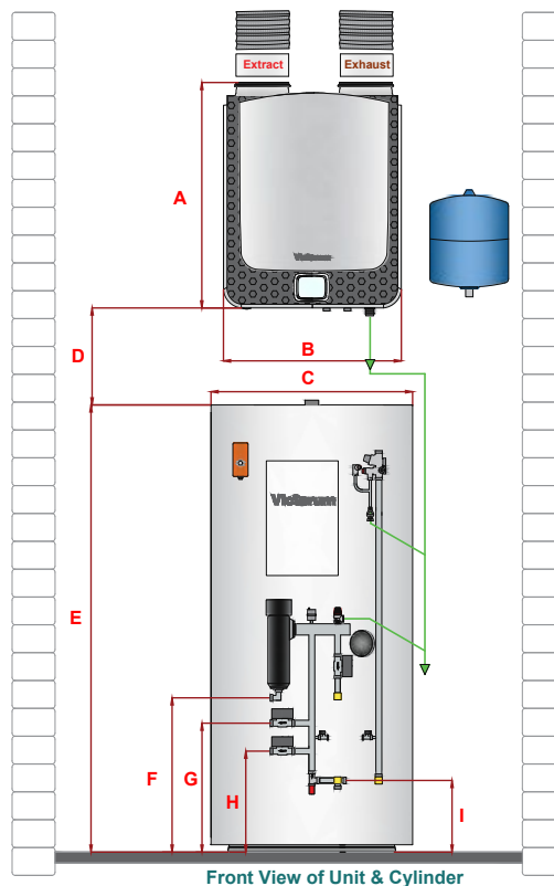
Front View of Unit & Cylinder
