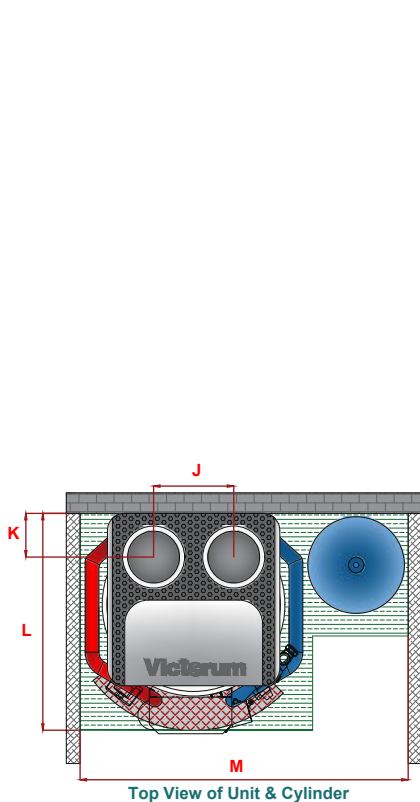
Top View of Unit & Cylinder
